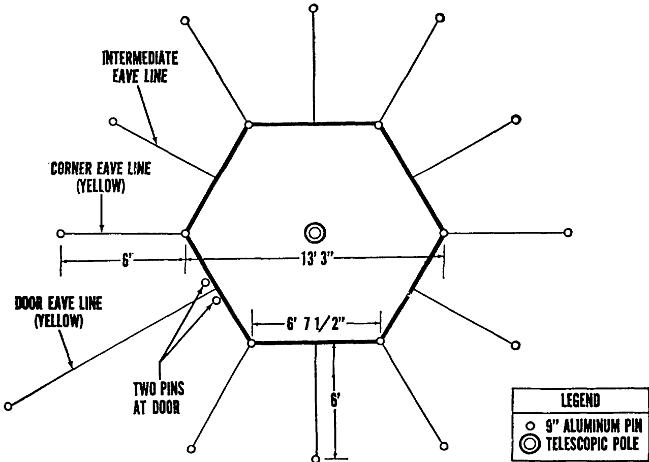
Figure 2-16. Ground plan, lightweight tent (M-1950).
